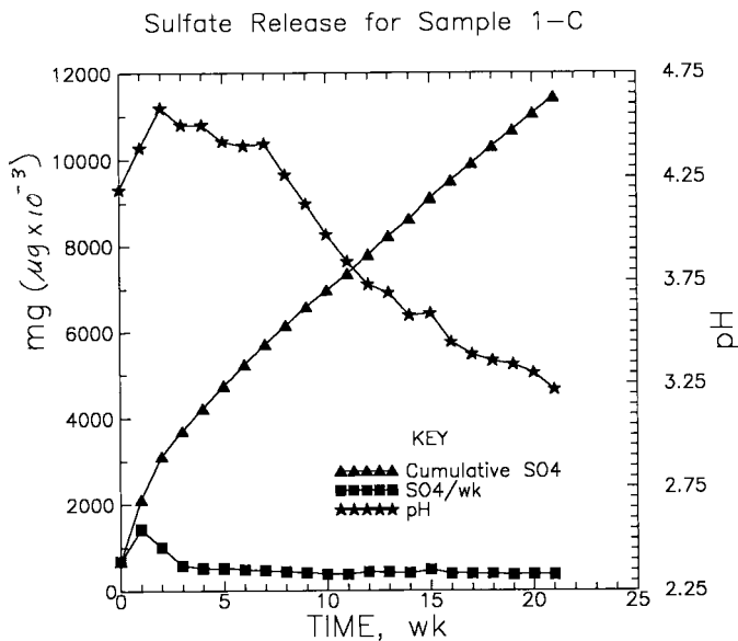
FIG. 5 Plot of Temporal Variation of pH, Sulfate Load, and Cumulative Sulfate from 21 Weeks
