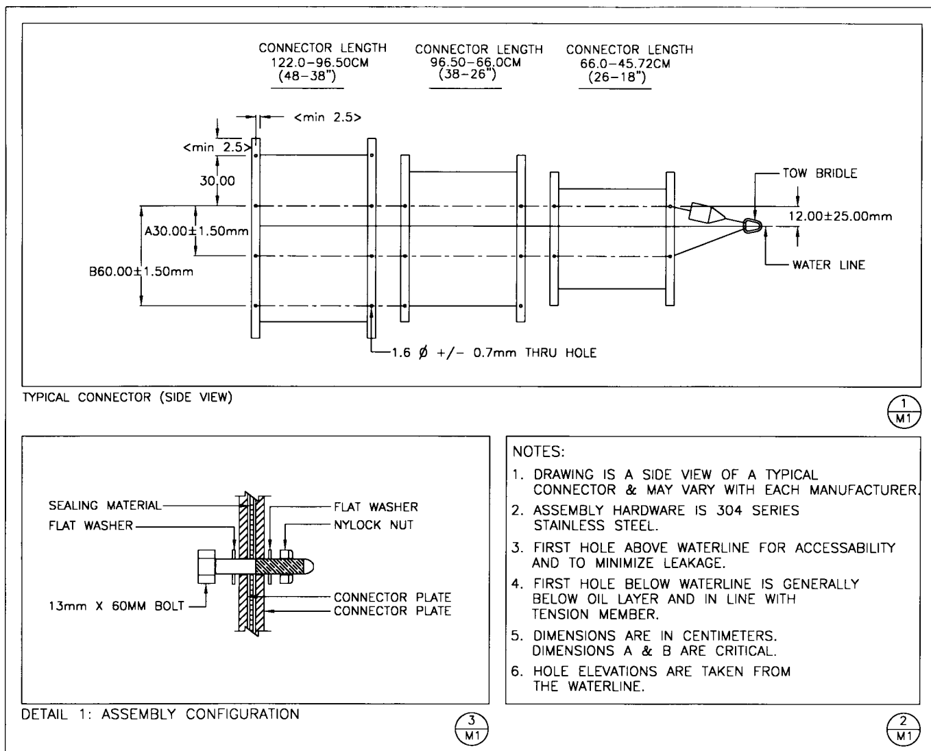
FIG. 1 Side View of a Typical Connector
