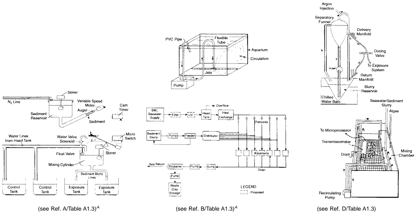
FIG. A1.2 Recirculating Tests
