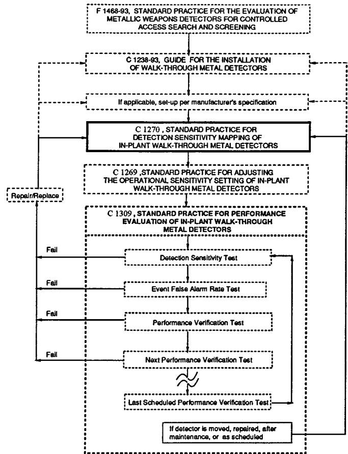
FIG. X1.1 Procedures for Walk-Through Metal Detector Program
