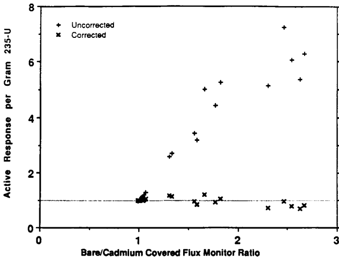
NOTE 1—The measured active response per gram of 235 U in 208-litre drums is shown for 20 matrices. Both the uncorrected response (+) and the flux monitor corrected response (x) are plotted. The standard deviation of the corrected responses is 14 %. The matrices have a wide range of characteristics typically found in facilities (2). The largest hydrogen content in a matrix was 9.65 kg; the largest boron content was 0.20 kg.
