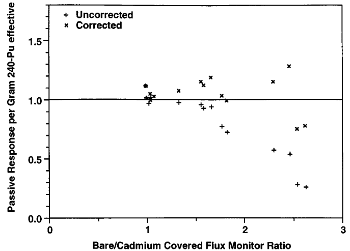
NOTE 1—The measured passive response per gram of 240 Pu effective is shown for 18 matrices. Both the uncorrected response (+) and the flux monitor corrected response (x) are plotted. The standard deviation of the corrected responses is 12 %. The matrices have a wide range of characteristics typically found in facilities (2). The largest hydrogen content in a matrix was 9.65 kg; the largest boron content was 0.20 kg.
