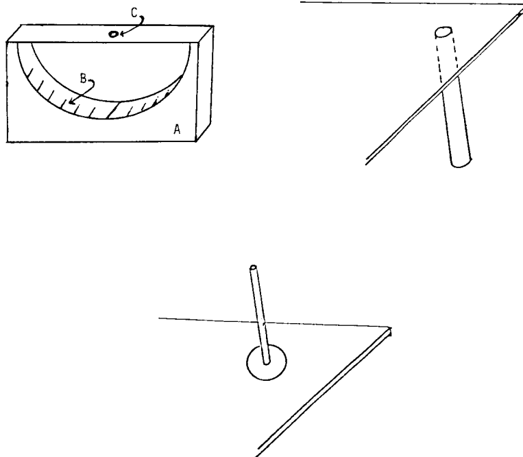
(a) Semicircle with scale (A) Semicircle with 143 mm radius cut out of 150 300 mm piece of 1/2 to 3/4 in. plywood. (B) Tape with 1 cm scale attached to inside of semicircle. (C) This opaque sheet (preferably metal) with 3 mm aperture centered above semicircle.
