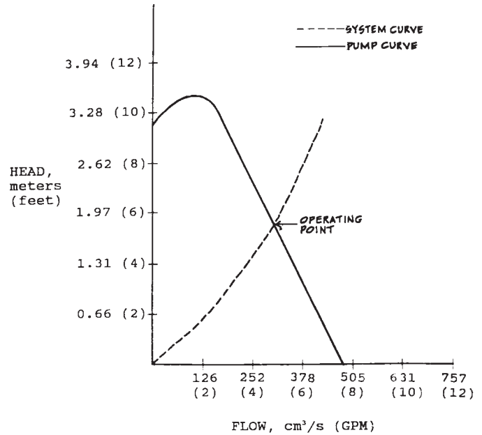
FIG. 2 Pump And System Curves (Closed Loop)
