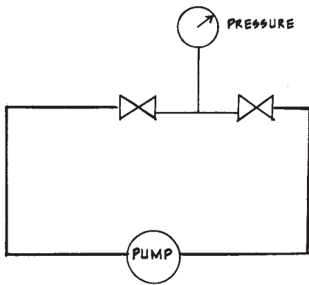
FIG. 4 Pressure Gage
