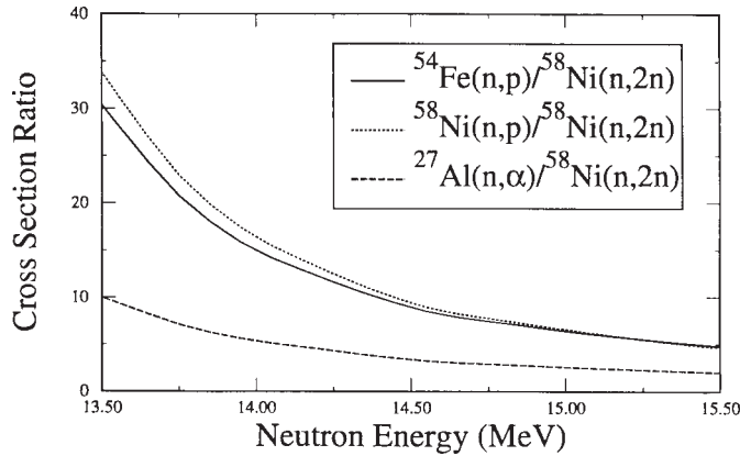
FIG. 7 Ratios of Cross Section for 3 H( d,n) 4 He Neutron Energy Determination
