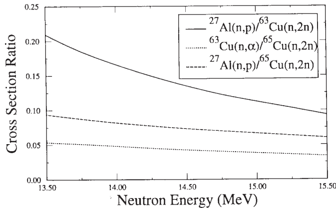
FIG. 8 Ratios of Cross Section for 3 H( d,n) 4 He Neutron Energy Determination
