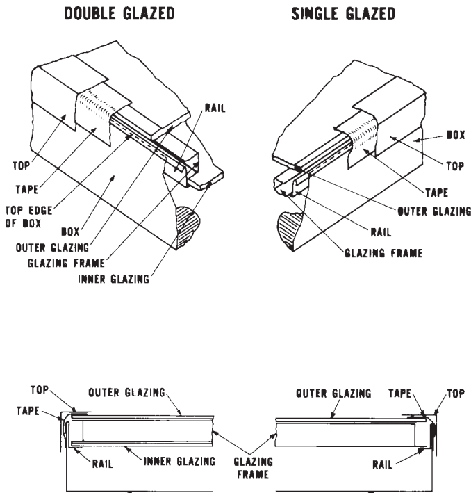
FIG. 5 Natural Weathering Box Assembly—Rigid Glazing
