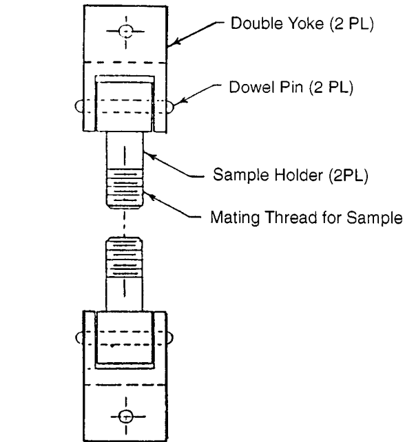
FIG. 2 Adaptor to Mate the Gripping Device to the Tensile Machine
