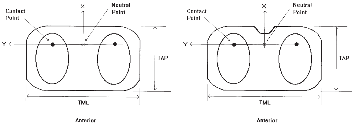
FIG. 5 ML Dimensions and Displacements Example
