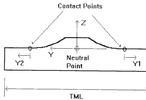
FIG. 5 ML Dimensions and Displacements Example
