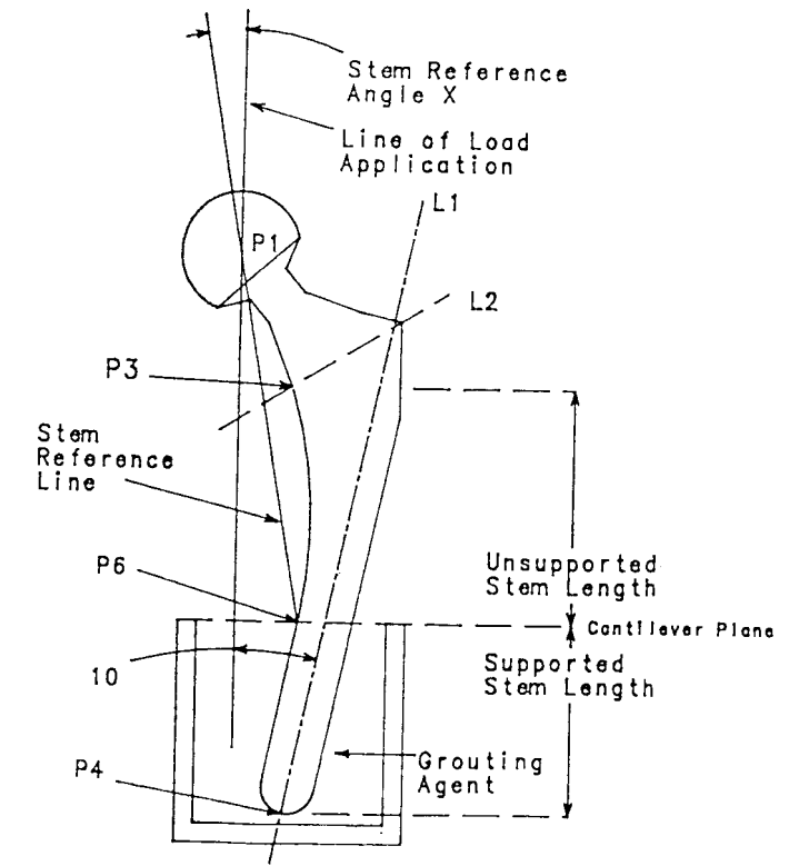
FIG. 2 1(b) Collarless Device, M-L Projection
