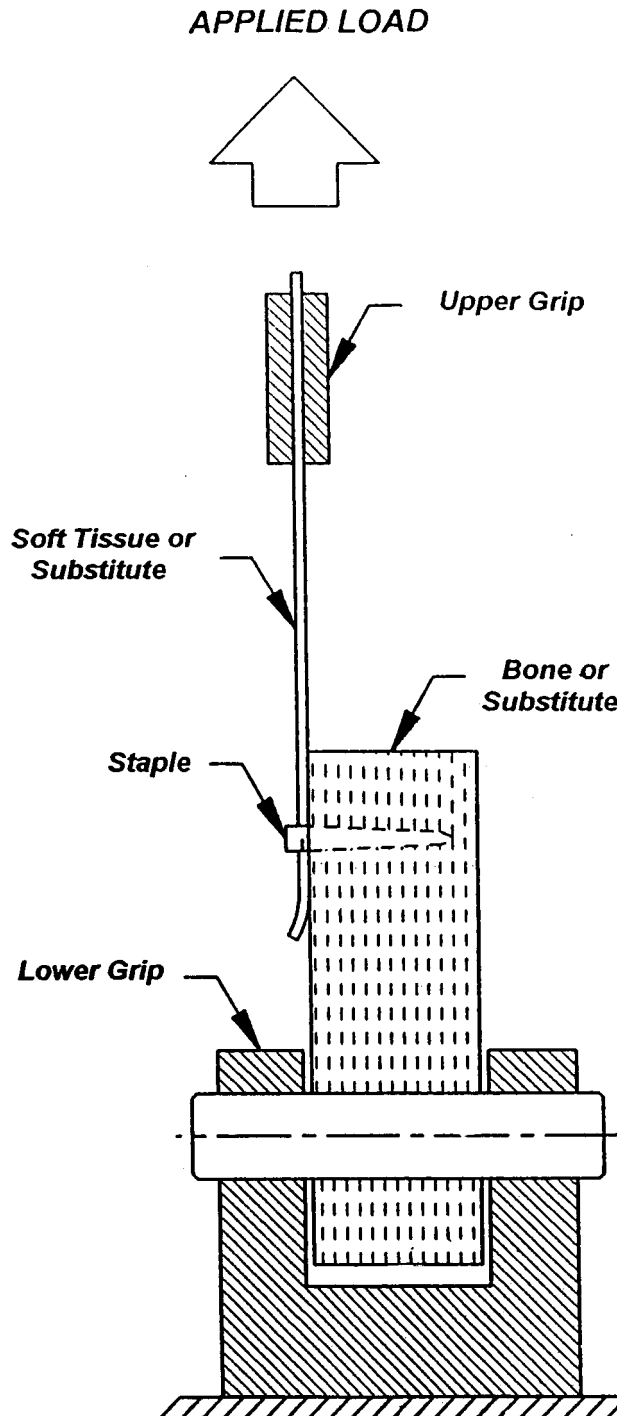
FIG. A3.1 Schematic of Tissue Fixation Strength Test
