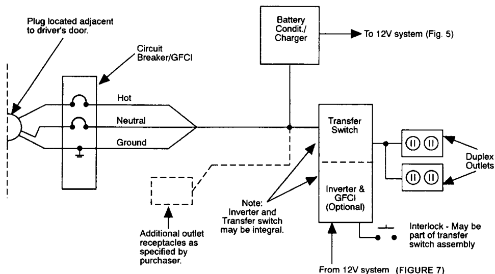
FIG. 8 115 Volt Electrical System - Functional Diagram
