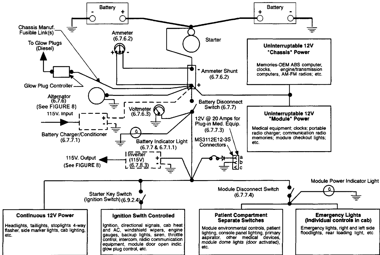
FIG. 7 12 Volt Electrical System - Functional Diagram
