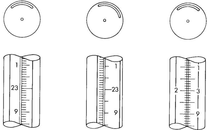
FIG. 14 Schemes for Graduation and Figuring
