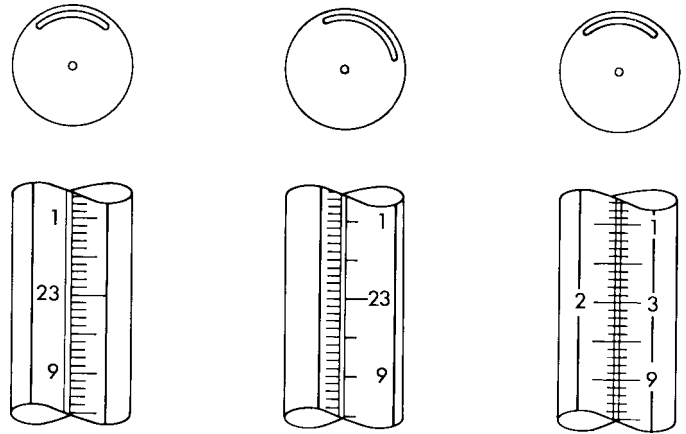
FIG. 14 Schemes for Graduation and Figuring
