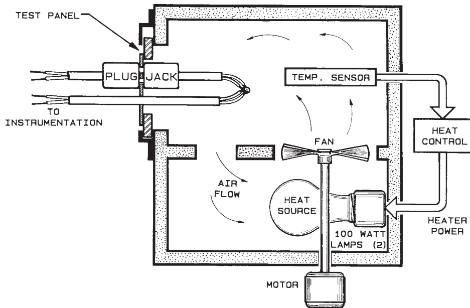
FIG. 2 General Arrangement for Thermal Gradient Test
