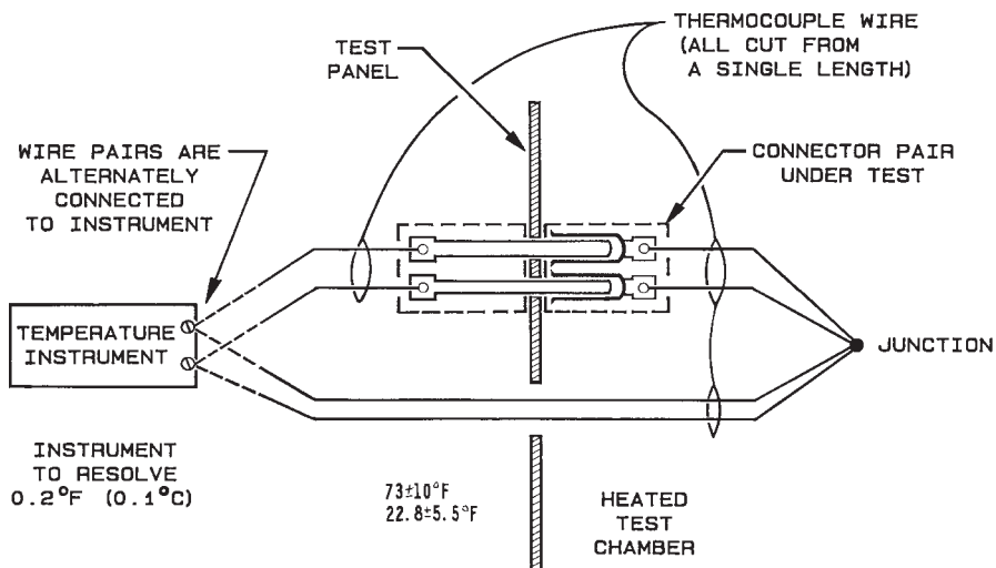
FIG. 3 Test Circuit for Thermal Gradient Test
