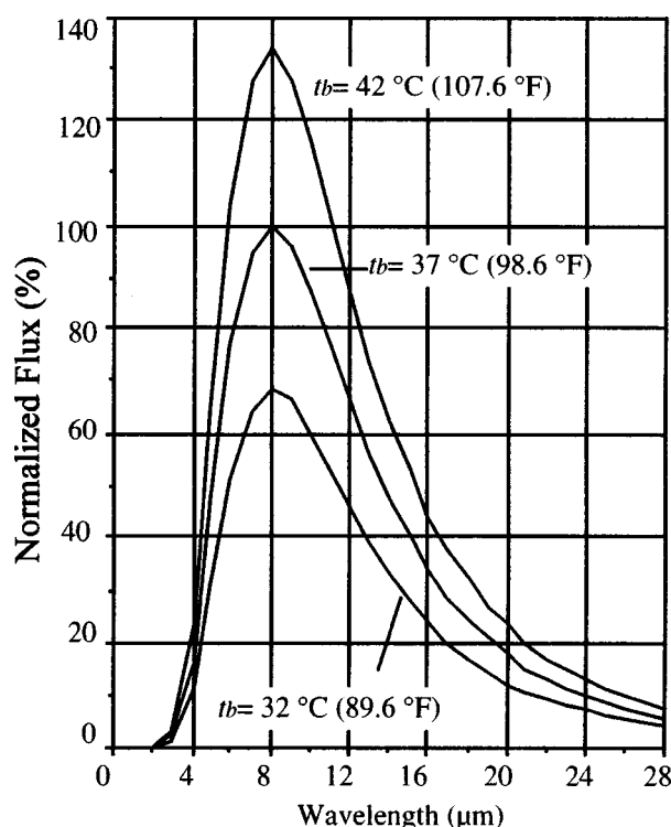
FIG. X1.1 Normalized with Respect to t_b=37 °C Spectral Net Flux Density for Three Blackbody Temperatures and IR Sensor at 20 °C (68 °F)
