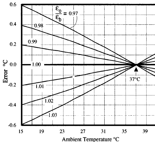
NOTE 1—Calculated for object's temperature of 37 °C, for various ratios of \epsilon_o/\epsilon_b .
