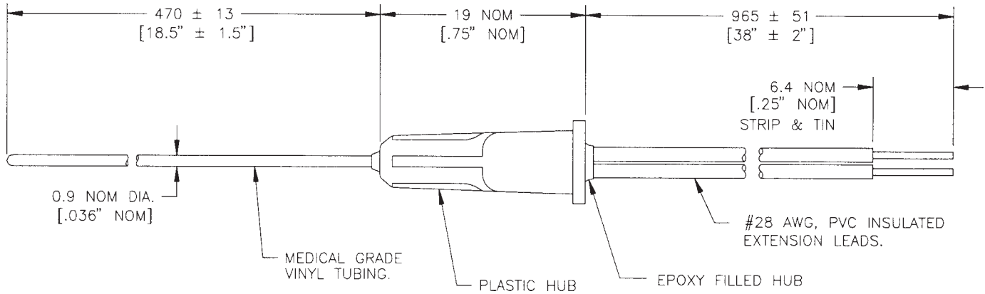
NOTE 1—Metric (English) All dimensions in millimetres unless otherwise indicated. FIG. 7 Non-Interchangeable Sensor Enclosed in 0.9 mm Vinyl Tube
