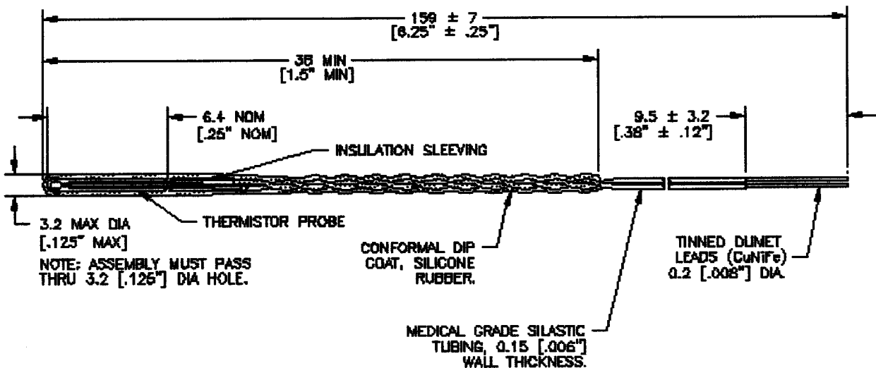
FIG. 2 Silicone Rubber Coated Glass Probe
