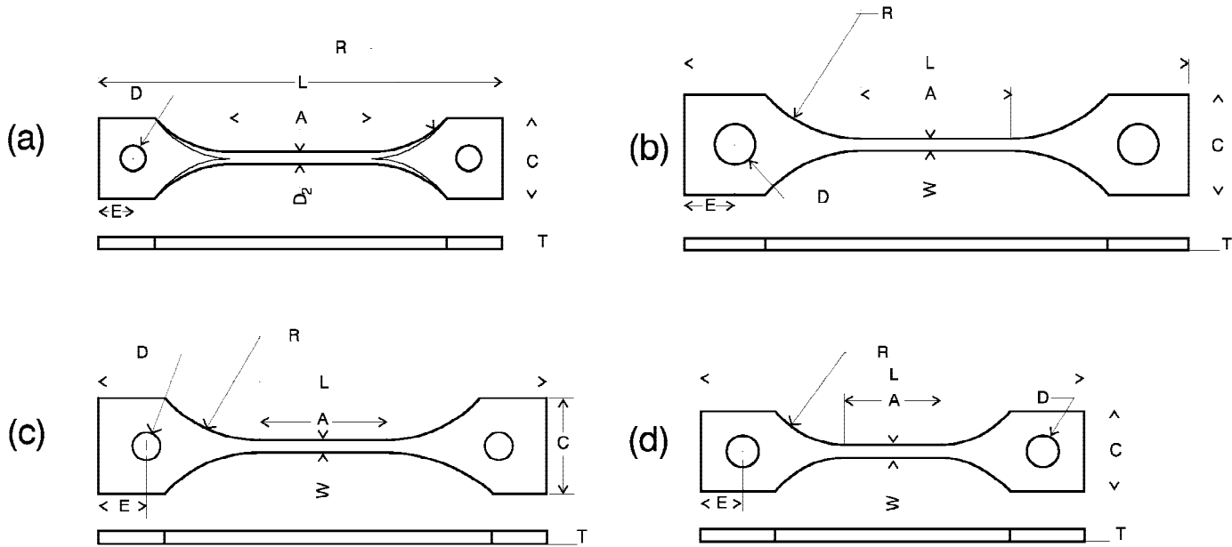
FIG. X1-2 Schematics of Typical Flat, Dogboned Specimens that have been Successfully Employed in Tensile Test Creep-Dep Experiments at Room Temperature.
