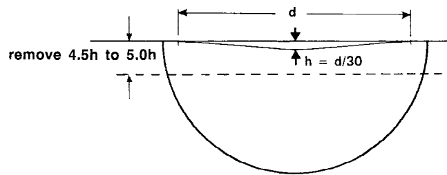
FIG. A3.54 The Precrack Extends Below the Knoop Hardness Impression, which has Depth, h
