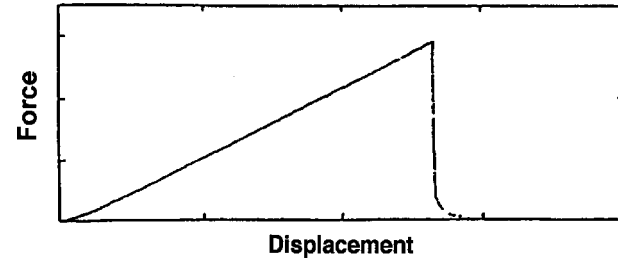
a) Unstable fracture from a chevron notch tip (invalid result) [34]
