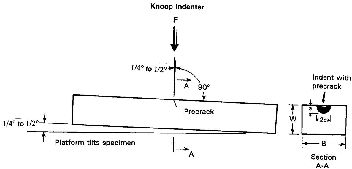
FIG. A3.2 Surface-Crack in Flexure (sc) Test Specimen
