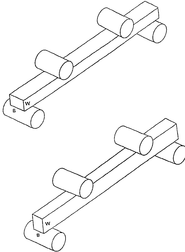
NOTE 1—The precrack must be on the tension (bottom) surface. FIG. A3.65 The Flexure Specimen Can be Tested with Either the Wide or Narrow Face on the Flexure Rollers
