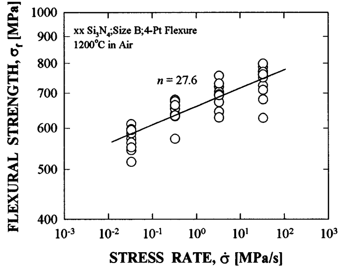
FIG. 5 Schematic of a Flexural Strength-Stress Rate Diagram, a Plot of \log(\text{Flexural Strength}) Versus \log(\text{Stress Rate})
