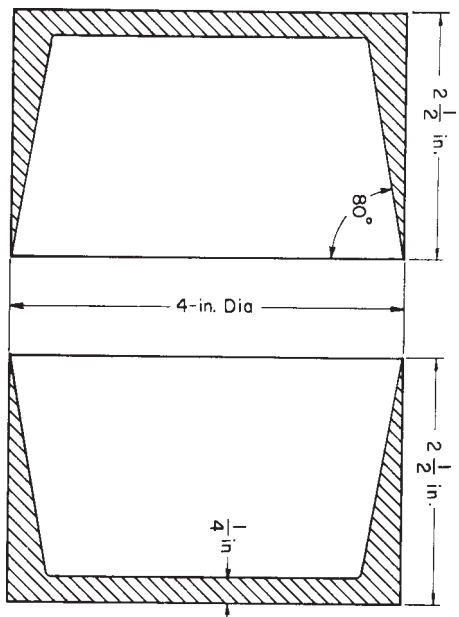
FIG. 2 Rubber Specimen-Sealing Gasket
