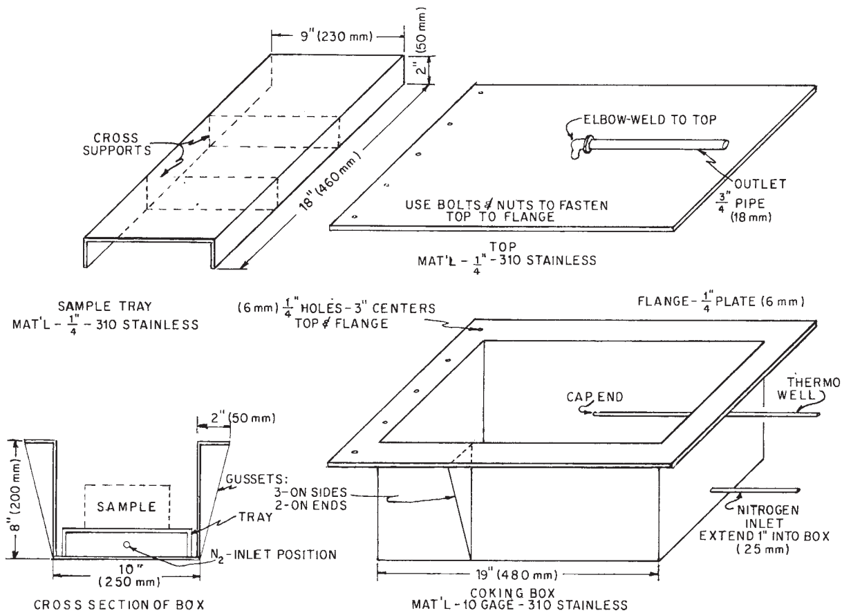
FIG. 1 Coking Box
