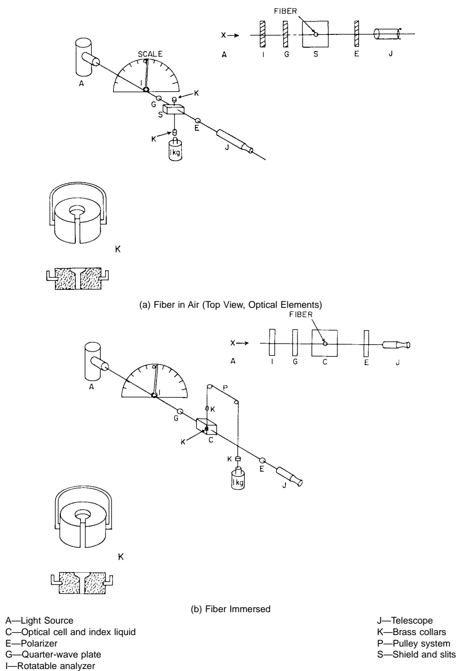
FIG. 3 Optical and Fiber-Stressing Polarimeter Arrangement
