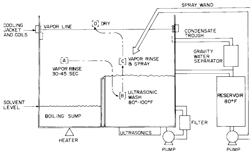
FIG. 1 Schematic of Vapor Cleaning System
