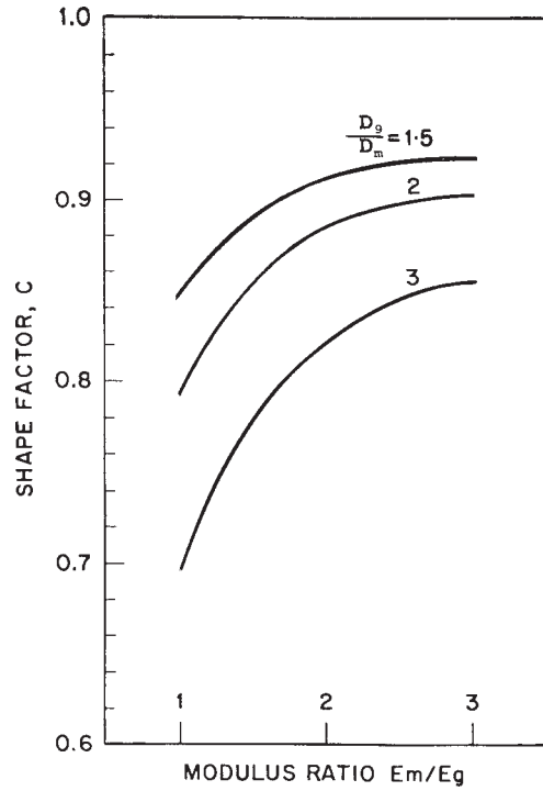
FIG. 1 Shape Factor, C—Modulus Ratio ( E_m/E_g ) Relationships for Three Glass/Metal Diameter Ratios
