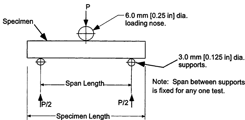
FIG. 6 Horizontal Shear Load Diagram (Flat Laminate)
