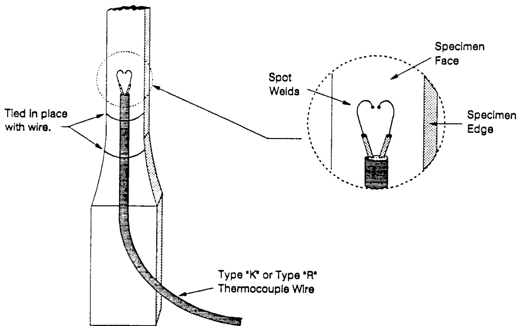
FIG. 4 Intrinsic (Spot Welded)
