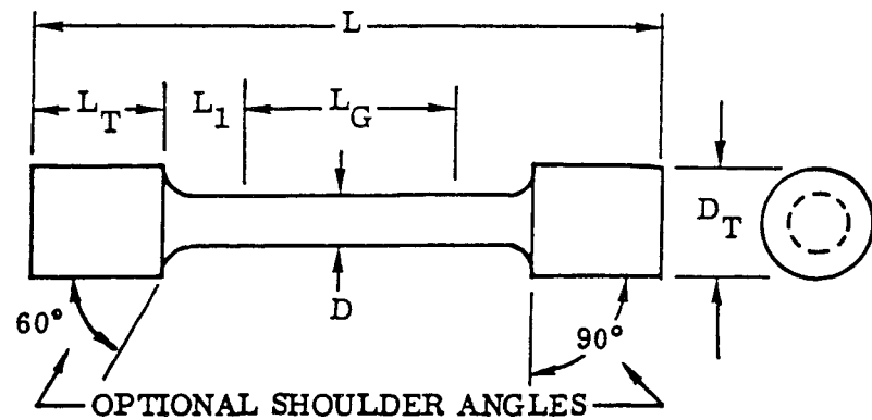
FIG. 2 Threaded Cylindrical Specimen (Dimensions in mm)
