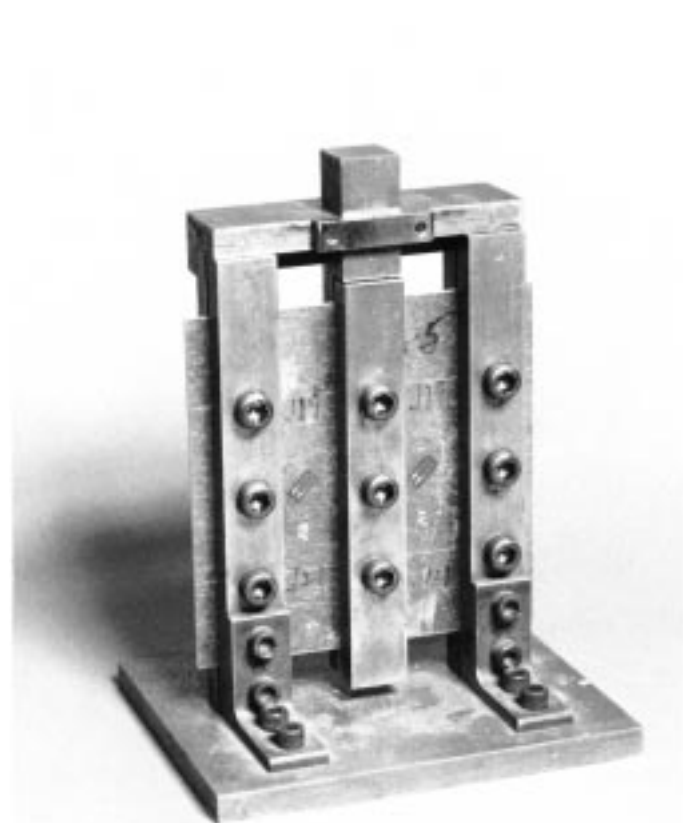
FIG. 2 Procedure A Partially Assembled Typical Test Fixture
