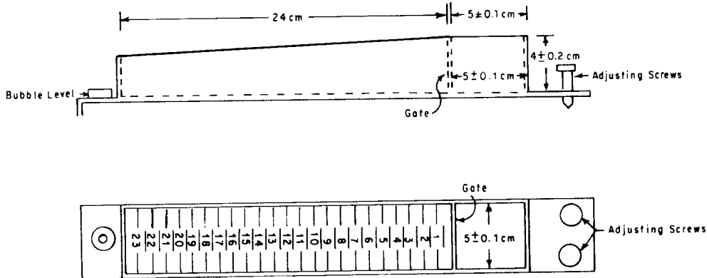
FIG. A1.1 Consistometer
