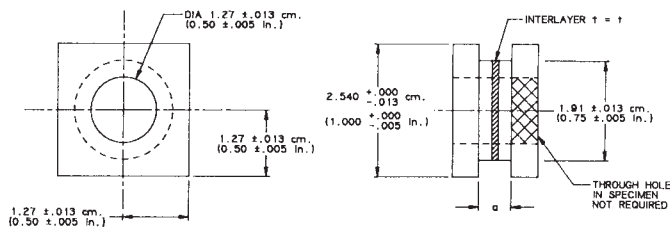
FIG. 4 Torsional Shear Test Specimen, Type I
