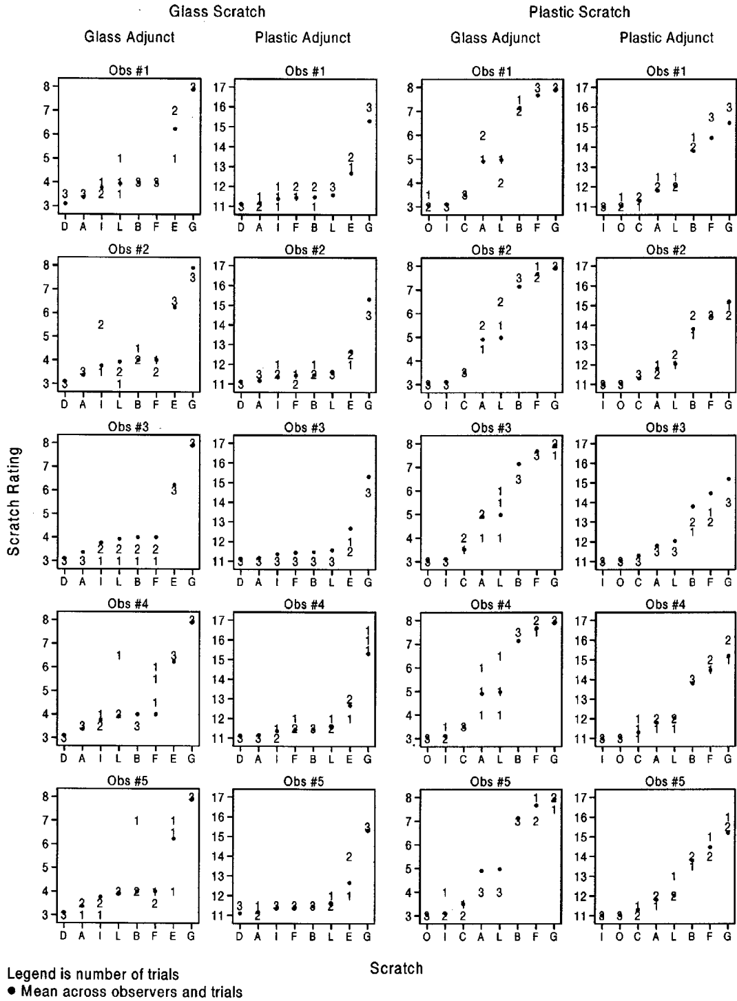
FIG. X1.32 Number of Trials for Each Observer and Scratch (N = 3) Having a Particular Scratch Rating when Compared with Either Glass or Plastic Adjunct
