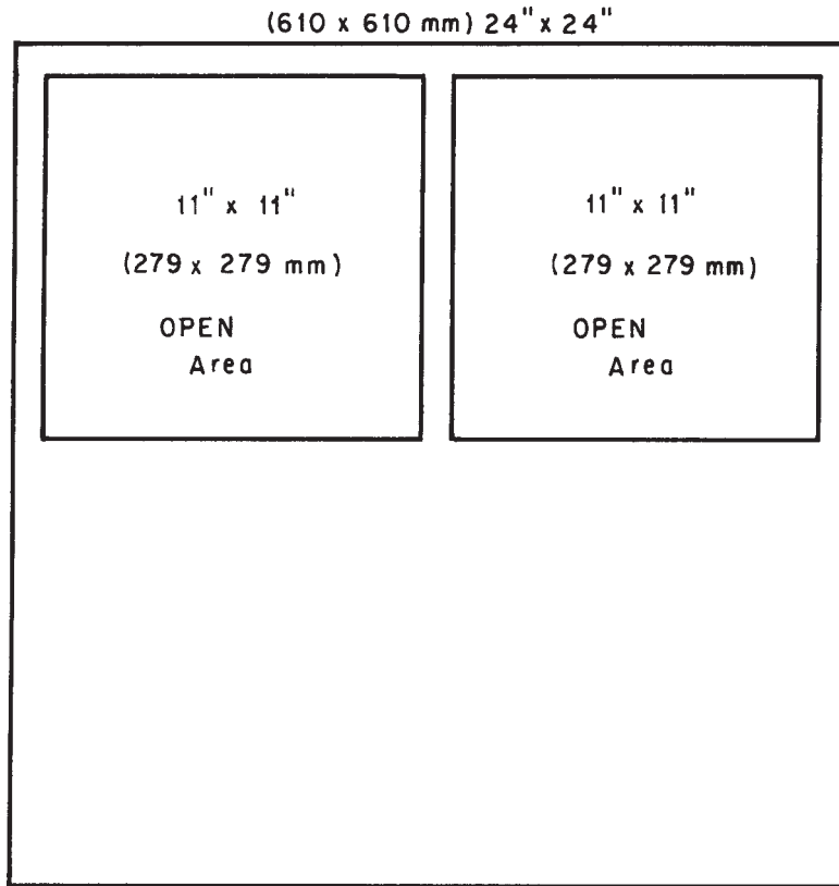
FIG. 2 Template, 24 by 24 in. (610 by 610 mm)
