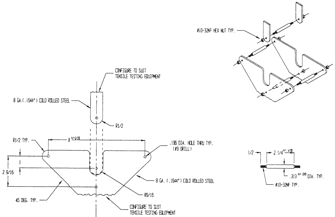
FIG. 1 Deflection Frame
