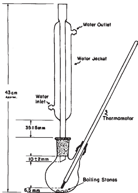
FIG. 1 Boiling Point Test Apparatus
