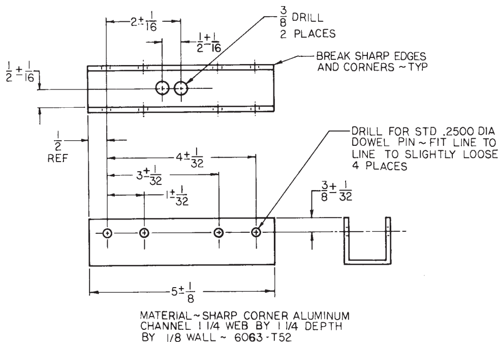
FIG. 3 Test Fixture Frame
