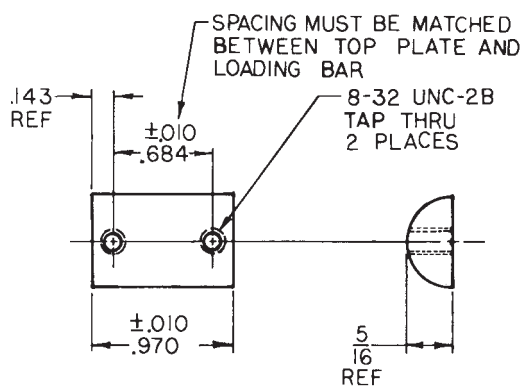
MATERIAL ~ 5/8 HALF-ROUND HOT ROLLED BAR FIG. 4 Test Fixture Center Loading Bar
