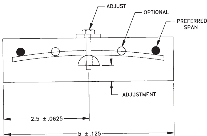
FIG. 6 Cut-Away View of Sample Mounted in Fixture
