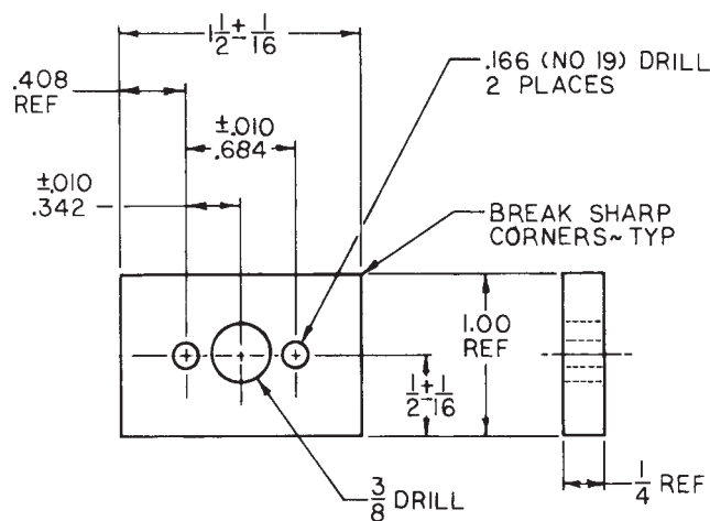
MATERIAL ~ 1/4 BY 1 COLD DRAWN FLAT FIG. 5 Test Fixture Top Plate
