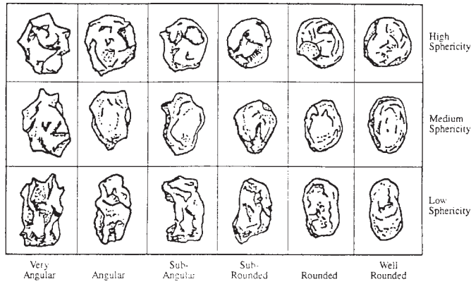
FIG. 1 Chart Showing the Angularity and Sphericity of Sand Grains
