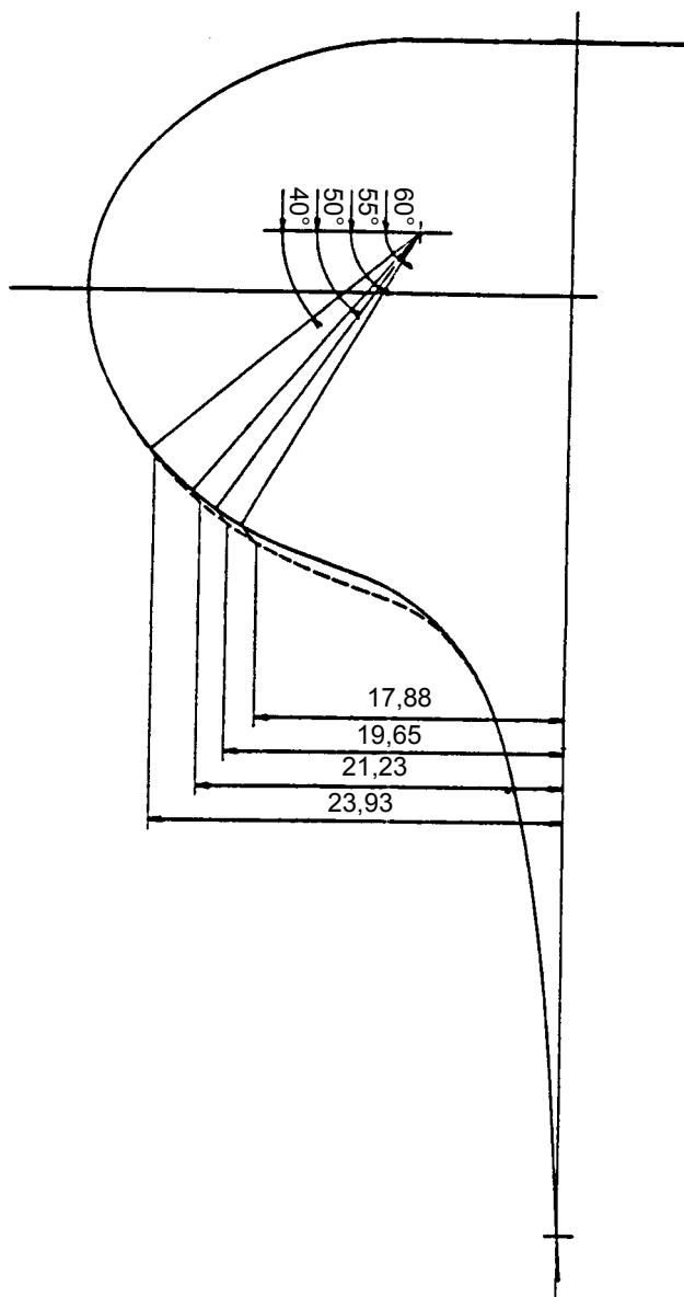
Fig. 5 - S1002 profile - Apparent contour - BOUTELOUP method
