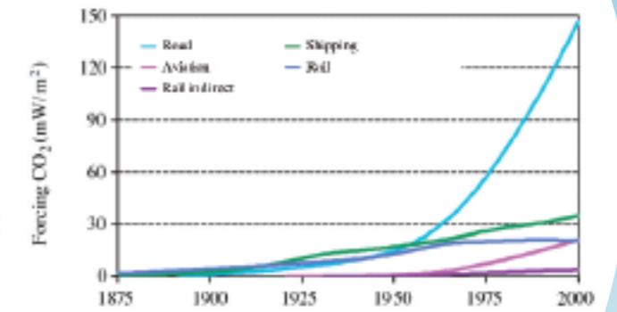
Source: Figure 1b in Fuglestvedt, J., T. Berntsen, G. Myhre, K. Rypdal and R. B. Skeie (2008). "Climate forcing from the transport sectors." Proceedings of the National Academy of Sciences of the United States of America 105(2): 454-458.
